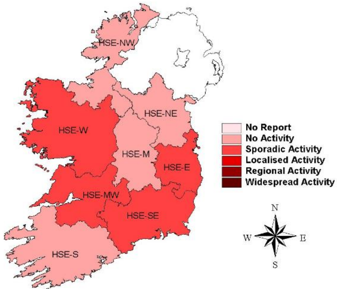
Figure 6: Map of provisional influenza activity by HSE-Area during week 14 2019
